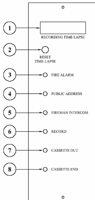
Figure 2-1 The cassette interface module front view
