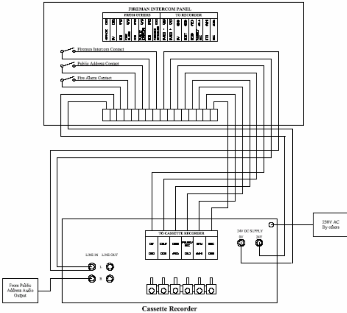
Figure 3-1 EVC7790 (Module) System connection & power supply setup
